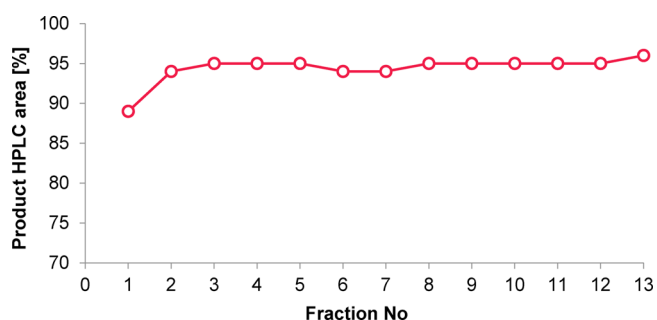
Figure 3. Product distribution of the steady-state experiment at a 1.3 M concentration of \alpha -tetralone (1). Fractions were collected at 7 min intervals.
